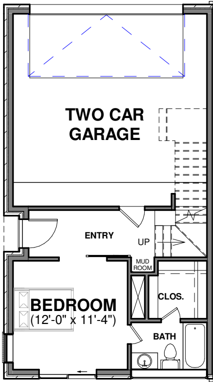
FIRST FLOOR 405 SF
