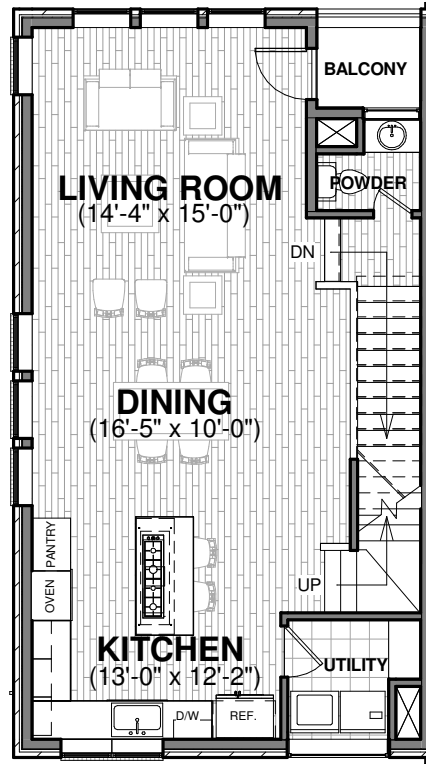
SECOND FLOOR 852 SF
