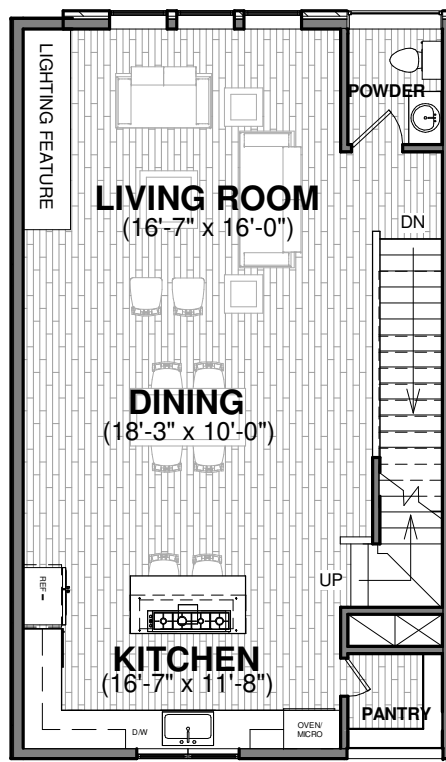
SECOND FLOOR 900 SF
