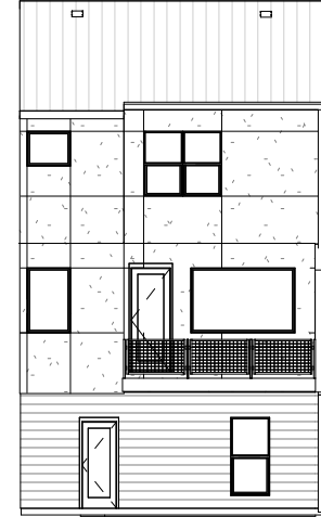
REAR ELEVATION
